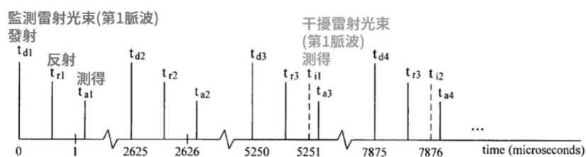
Fig. 1 (Prior Art)
