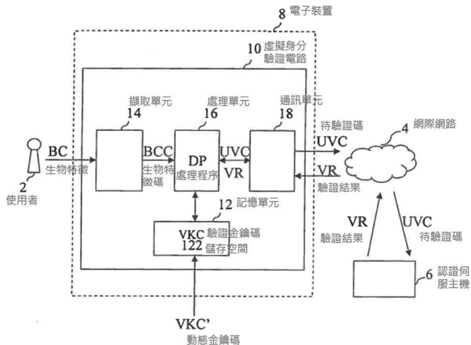
附圖 1 一系爭專利之虛實身分驗證電路的方塊示意圖
