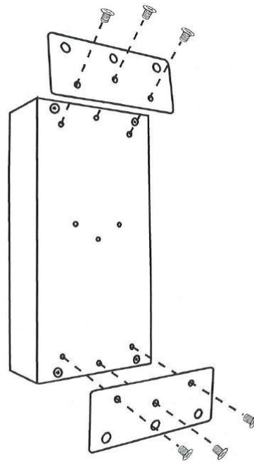
Figure 2.2 Attaching the Metal Mounting Kit
