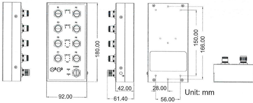
Figure 2.1 EKI-6528TI/6528TPI Dimensions
