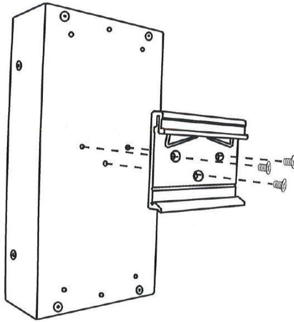
Figure 2.3 DIN-rail Installation
