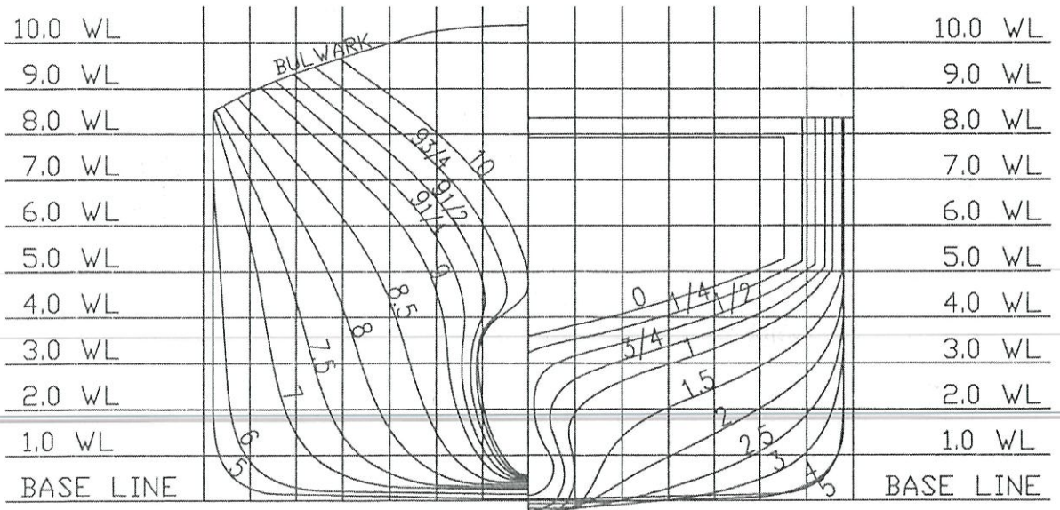
BODY PLAN SCALE : 1/75
