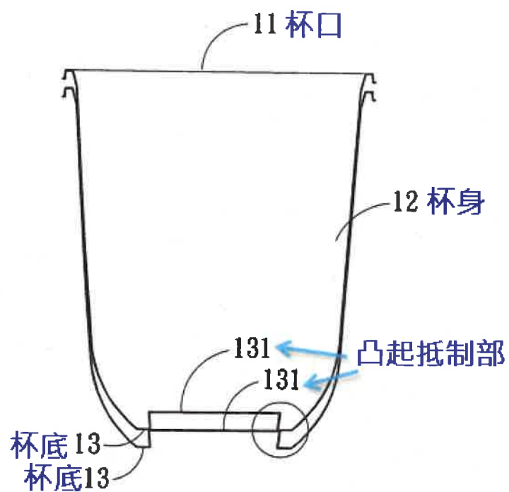
第八圖係為系爭專利之杯體堆疊局部結構示意圖
