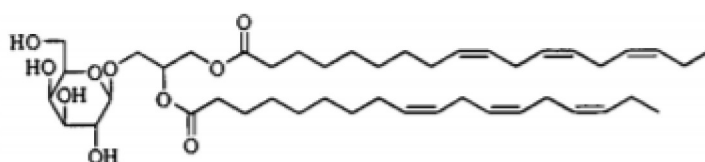
1,2-二-O- \alpha -次亞麻油醯基-3-O- \beta -半乳糖吡喃糖基-sn-甘油(1,2,di-O- \alpha -linolenoyl-3-O- \beta -galactopyranosyl-sn-glycerol, dLGG)
