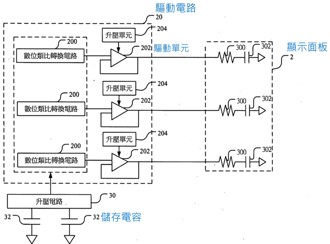
系爭專利之驅動電路的電路圖
